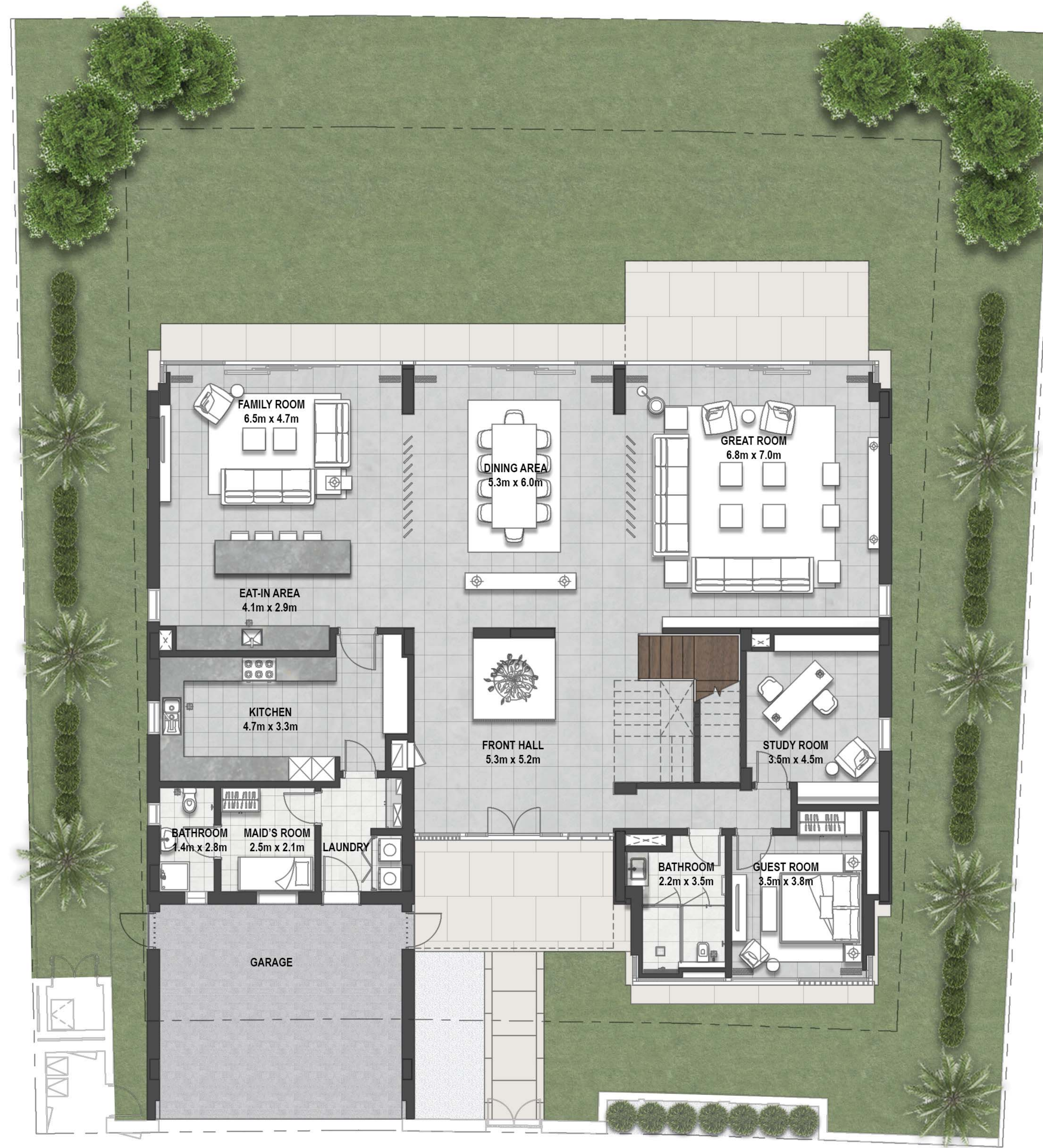
GROUND FLOOR
