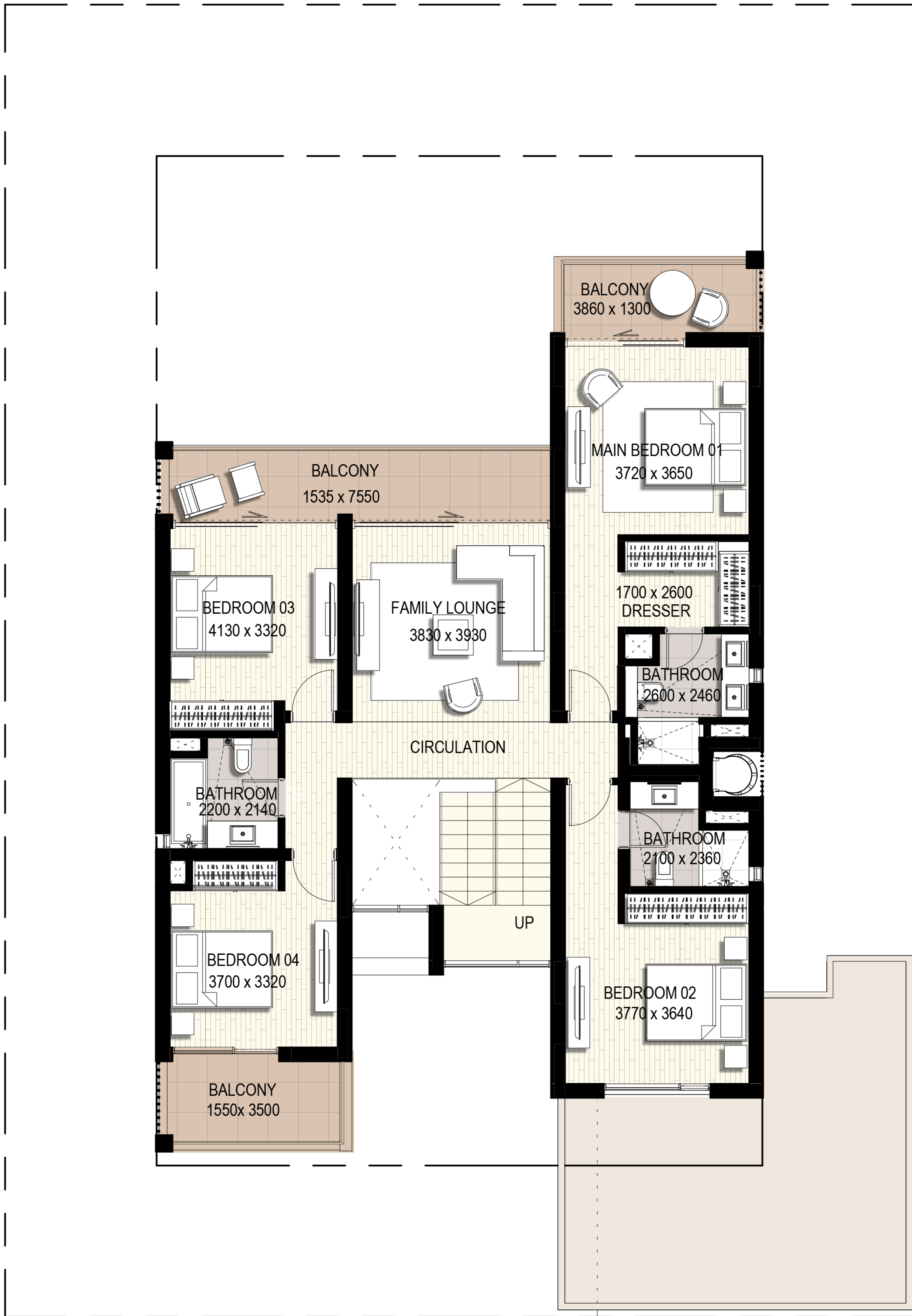
First Floor
